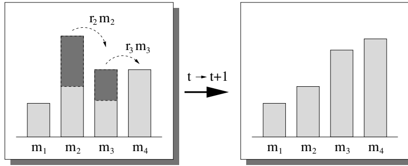
Figure 1. Mass representation of the ARAP with parallel dynamics. The height of a mass stick corresponds to m_i . The fragments r_i m_i are shaded.
